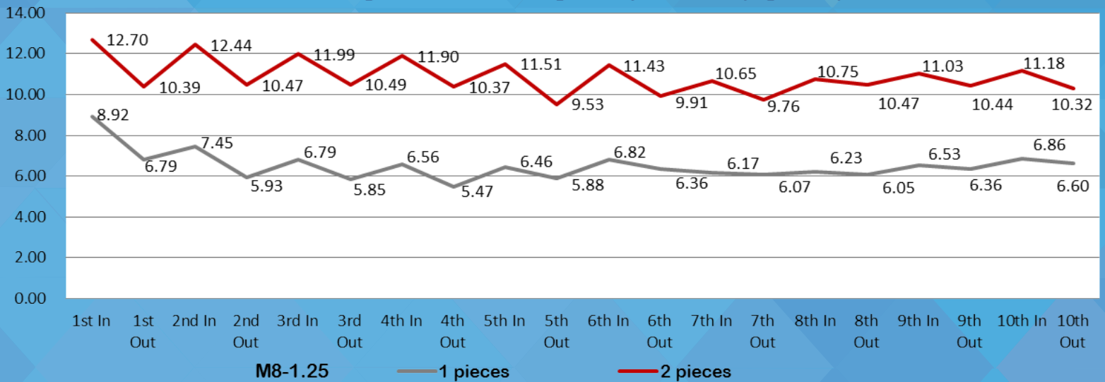
Self Locking Nut Prevailing Torque Test (kgf.cm)
